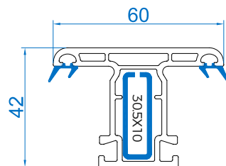
Sash Mullion - 42 RSM-42SM Mtr Wt :-0.744
