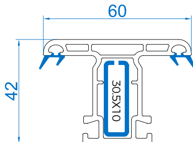
Sash Mullion - 42 RSM-42SM Mtr Wt :-0.744
