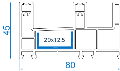
2.5 Track - 80 Series RSMT-80ET Mtr Wt :-1.191
