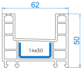
2 Track - 62 RSMT-62T Mtr Wt :-0.960
