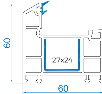
Casement Outer - 60 RSMC - 60 OF Mtr Wt :-1.047
