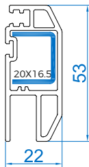
Mesh - 53 RSMM-53M Mtr Wt :-0.502
