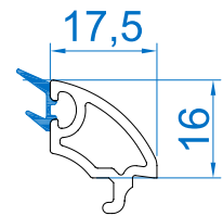
Bead - 17.5 RSMB - 17.5EB Mtr Wt :-0.195
