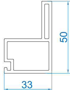
Add On Track
