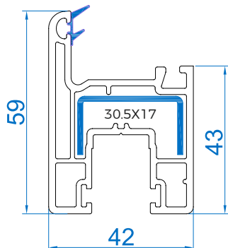
Small Sash - 59 RSMS-59SS Mtr Wt :-0.876
