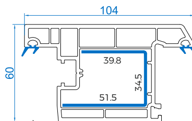
Casement Outward Door Sash RSMC - 104 OD Mtr Wt :-1.559
