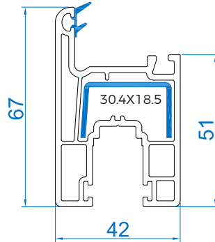
Medium Sash - 67 RSMS-67MS Mtr Wt :-0.972
