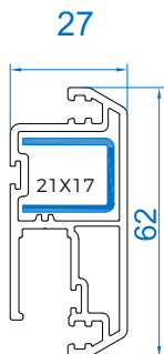
Mesh Mullion - 62 RSMM-62MM Mtr Wt :-0.610
