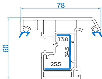
Outward Window Sash - 78 RSMC - 78 WO Mtr Wt :-1.255
