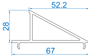
Corner Joint Copular - 112
