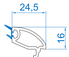
Bead - 24.5 RSMB-24.5SB Mtr Wt :-0.259
