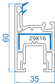
Sash - 60X35 RSMS-60ES Mtr Wt :-0.786
