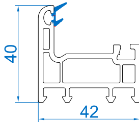
Small Casement Frame - 42 RSMC - 42 VF Mtr Wt :-0.585
