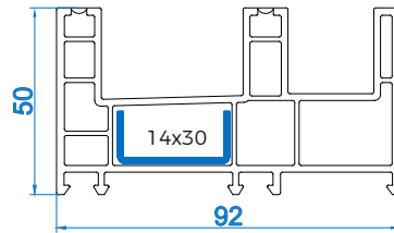
2.5 Track - 92 RSMT-92T Mtr Wt :-1.329
