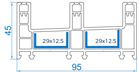
3 Track - 95 Series RSMT - 95ET Mtr Wt :-1.356
