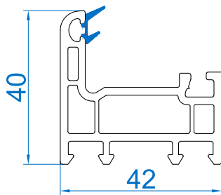
Small Casement Frame - 42 RSMC - 42 VF Mtr Wt :-0.585
