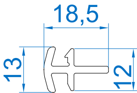
H Coupler
