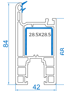
Big Sash - 84 RSMS-84BS Mtr Wt :-1.220
