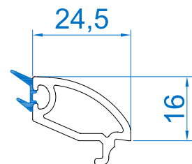
Bead - 24.5 RSMB-24.5SB Mtr Wt :-0.259
