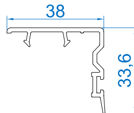
Interlock - Small RSMI - 38EIL Mtr Wt :-0.202
