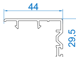
Inter Lock - 44 RSMI-44IL Mtr Wt :-0.220
