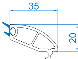
Casement Big Bead - 35 RSMC - 35 CB Mtr Wt :-0.353
