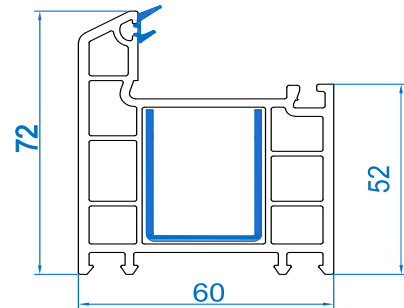
Casement Outer - 72 RSMC - 72 OF Mtr Wt :-1.246
