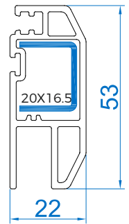
Mesh - 53 RSMM-53M Mtr Wt :-0.502
