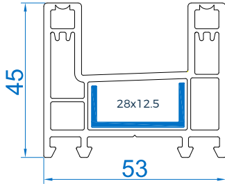
2 Track - 53 RSMT-53ET Mtr Wt :-0.835
