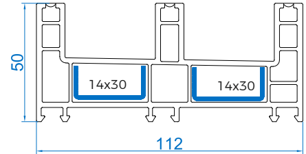
3 Track - 112 RSMT-112T Mtr Wt :-1.704
