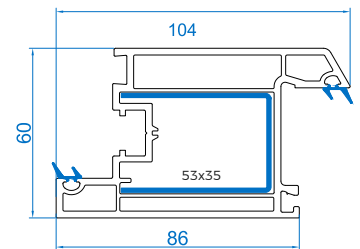
Casement Inward Door Sash RSMC - 104 ID Mtr Wt :-1.621
