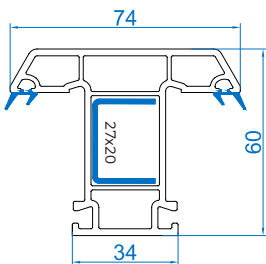
T - Mullion - 74 RSMC - 74TM Mtr Wt :-1.071
